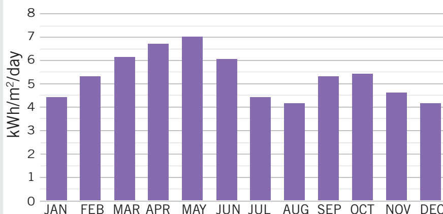
Figure 21: Annual Solar Irradiance of the site
